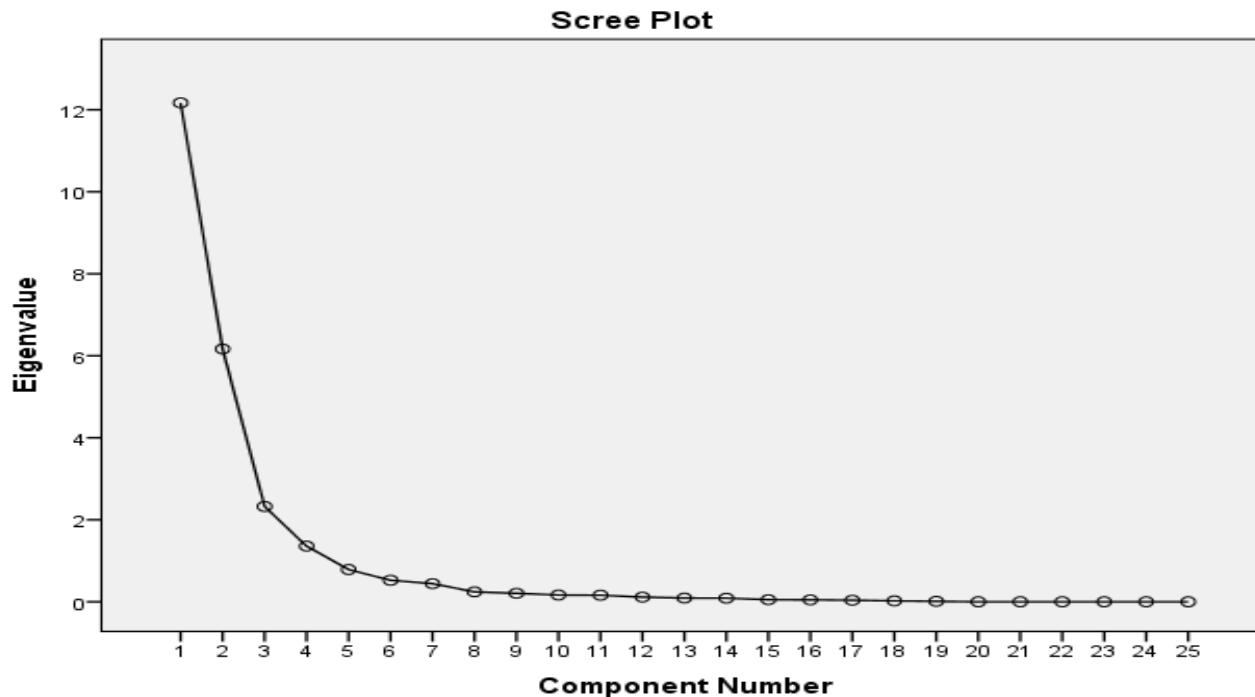
Fig 4.1: Scree Plot
